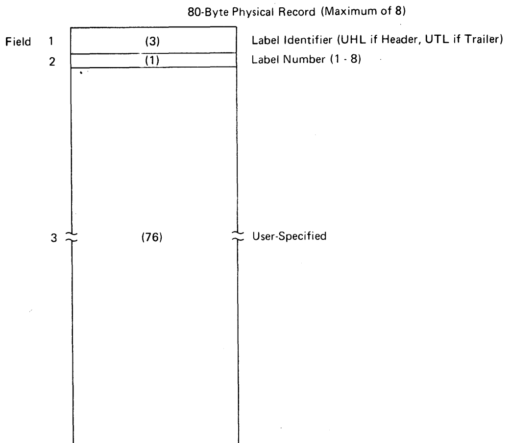
Figure 73. User Header and Trailer Labels
