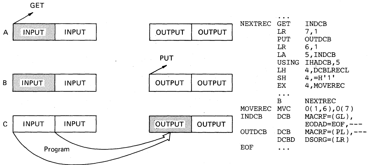
Figure 35. Simple Buffering with MACRF=GL and MACRF=PL
