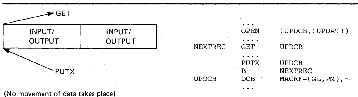
Figure 36. Simple Buffering with MACRF=GL and MACRF=PM-UPDAT Mode
