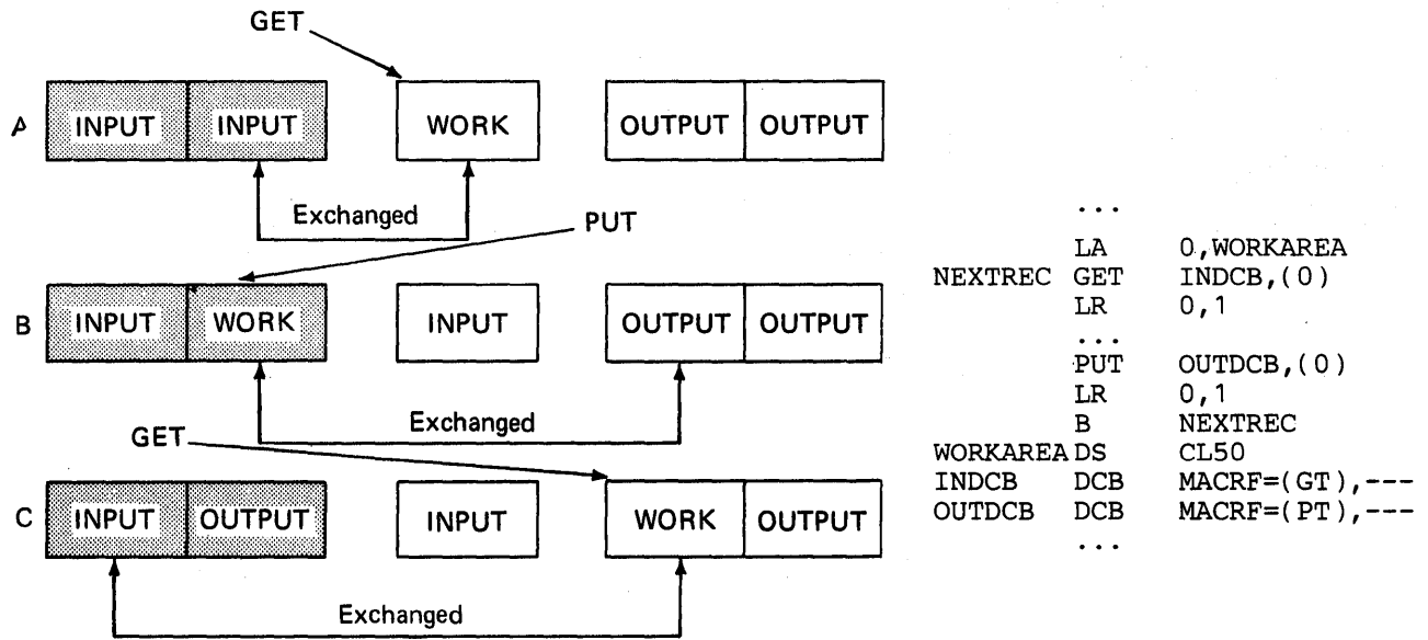
Figure 37. Exchange Buffering with MACRF=GT and MACRF=PT
