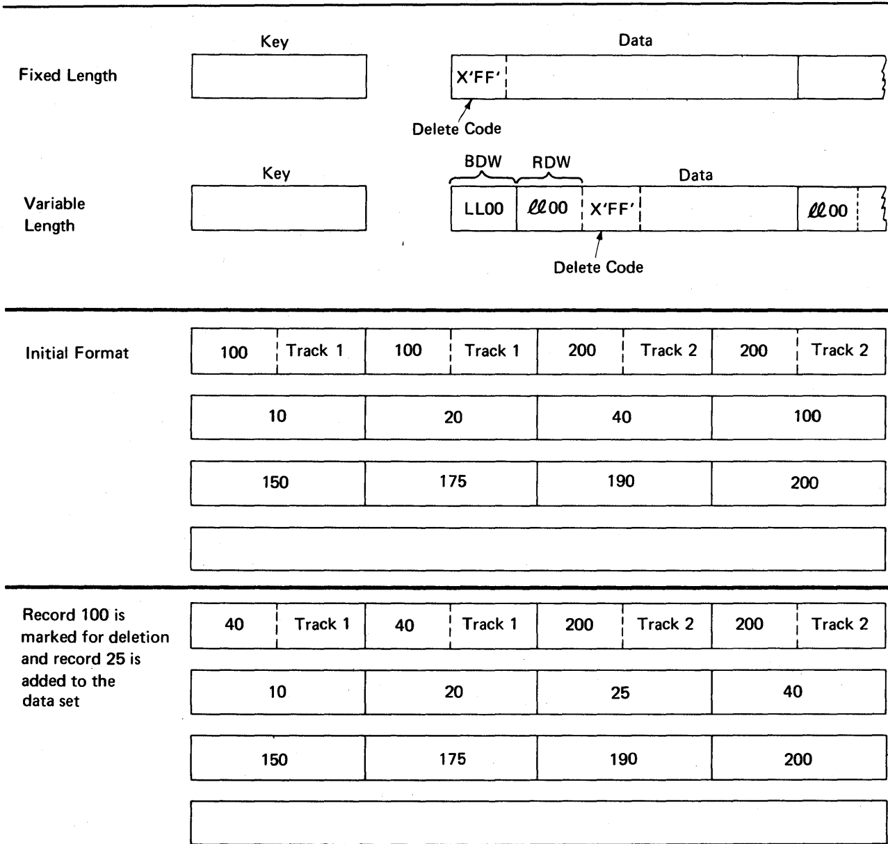
Figure 58. Deleting Records From an Indexed Sequential Data Set
