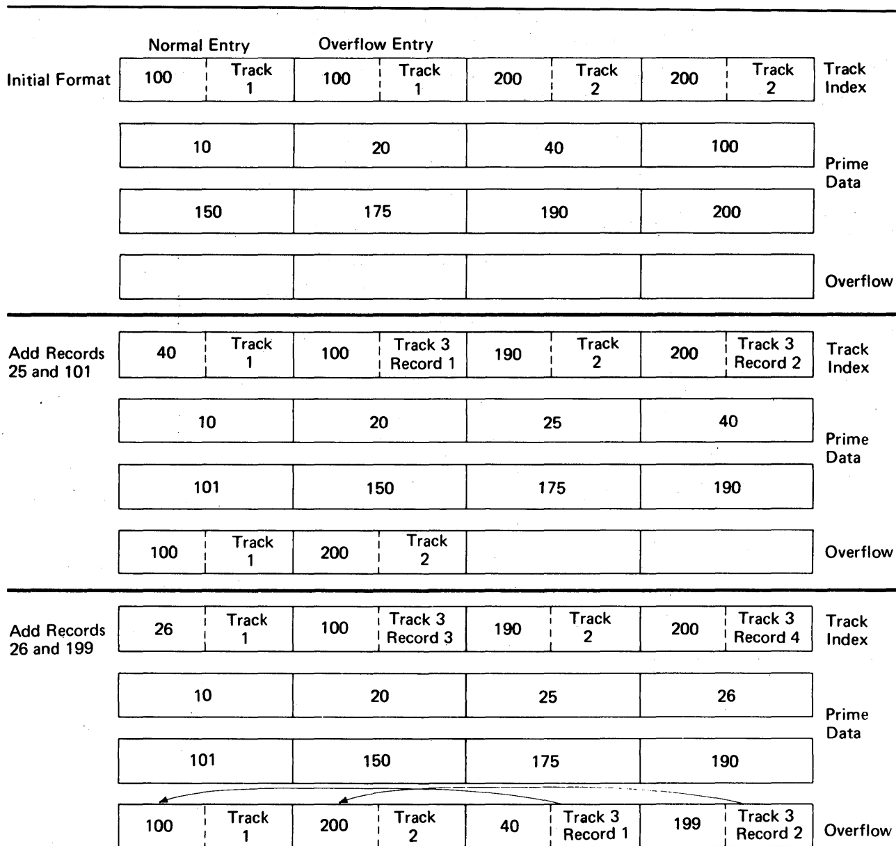
Figure 57. Adding Records to an Indexed Sequential Data Set
