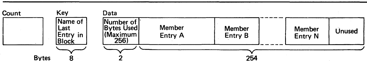
Figure 47. A Partitioned Data Set Directory Block
