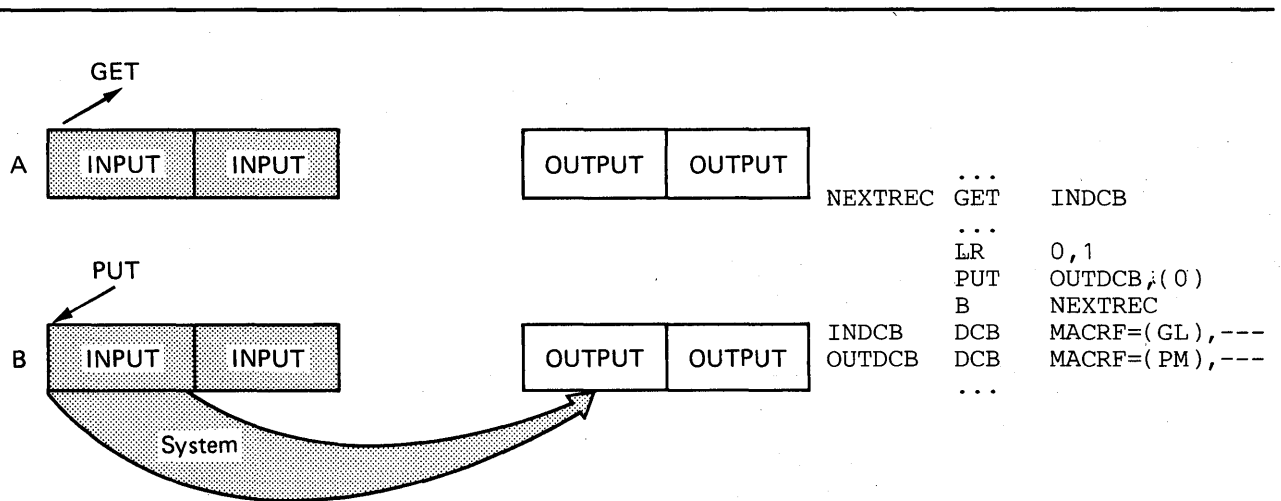
Figure 33. Simple Buffering with MACRF=GL and MACRF=PM
