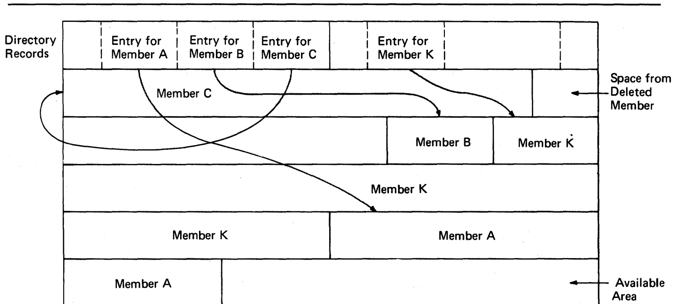
Figure 46. A Partitioned Data Set
