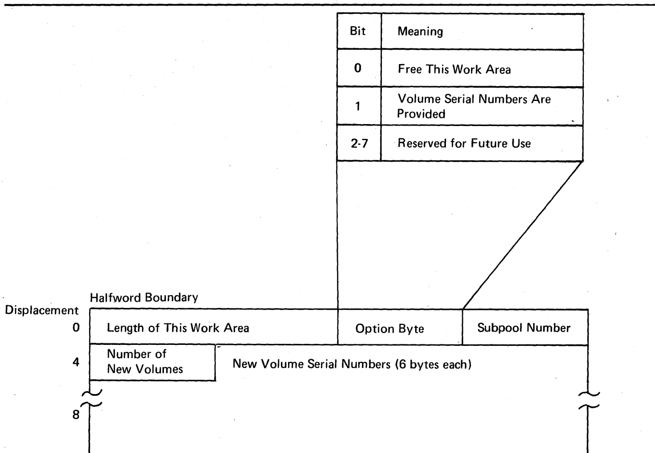
Figure 22. Recovery Work Area
