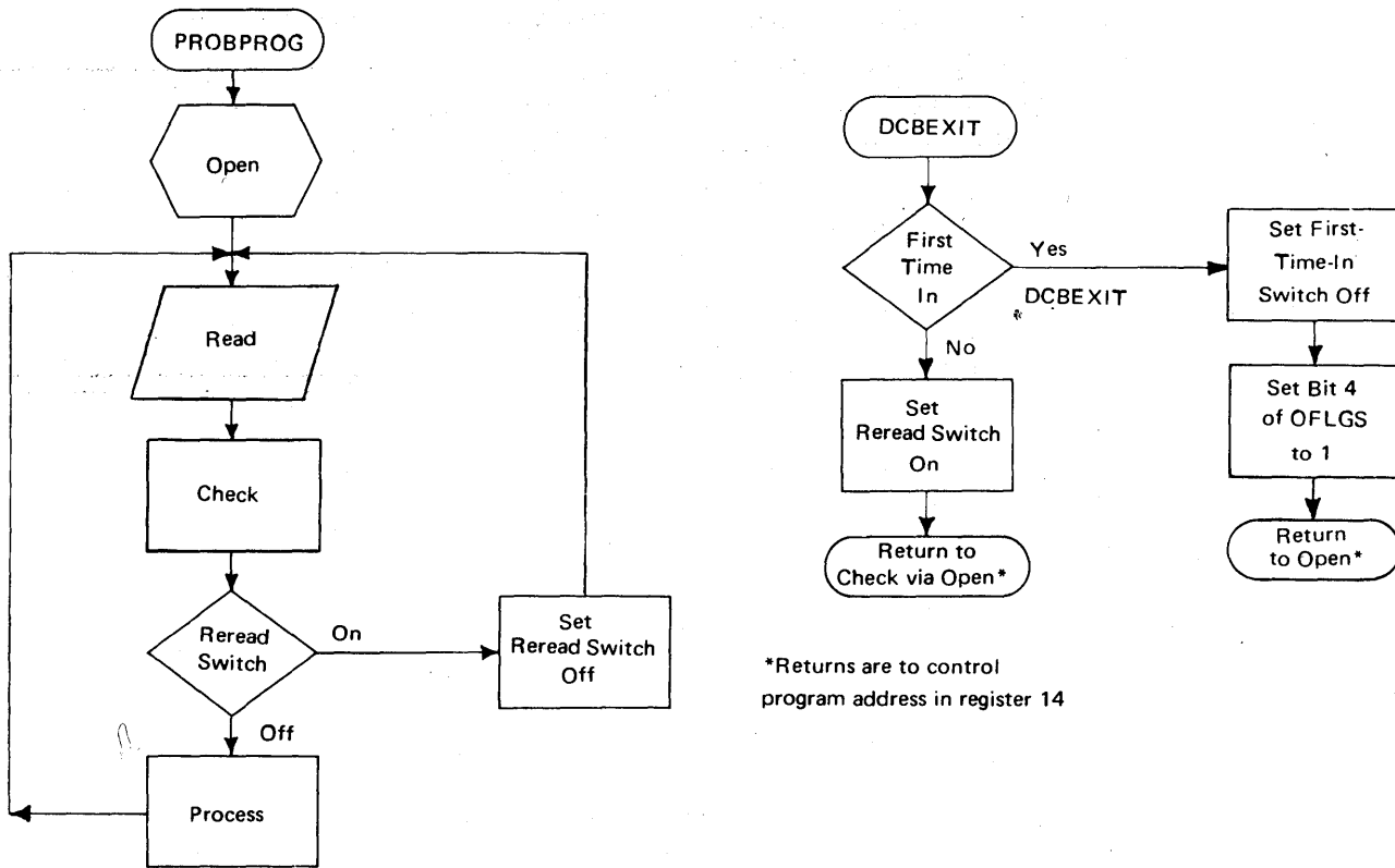
Figure 69. Reissuing a READ for Unlike Concatenated Data Sets
