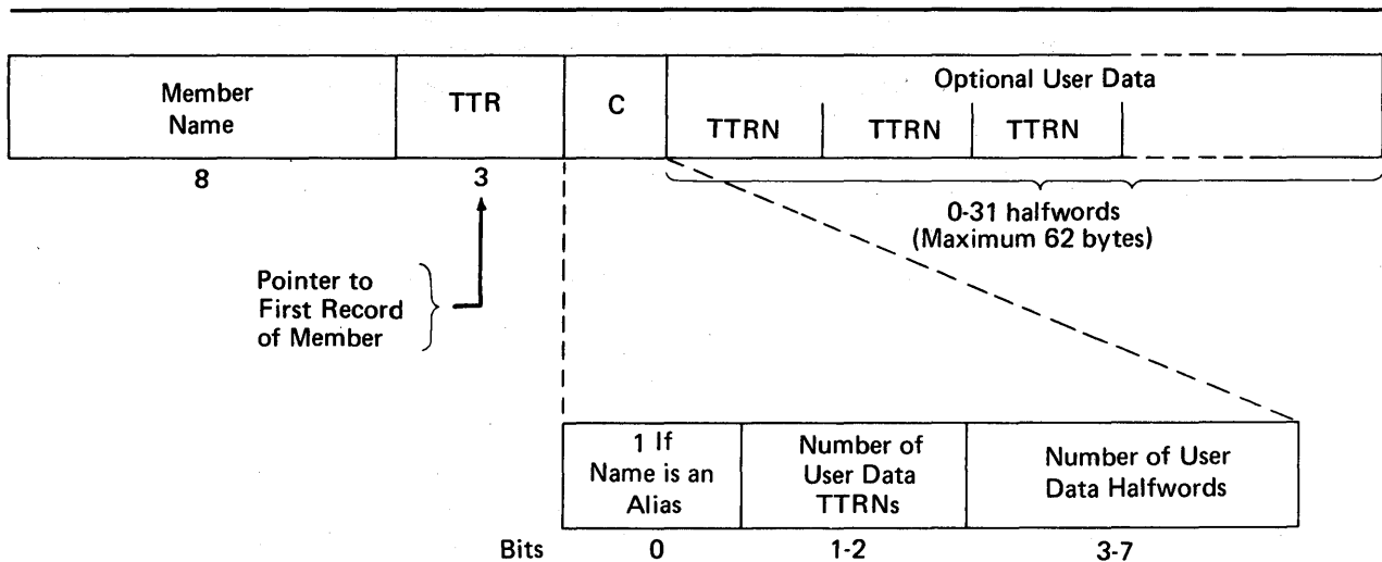
Figure 48. A Partitioned Data Set Directory Entry
