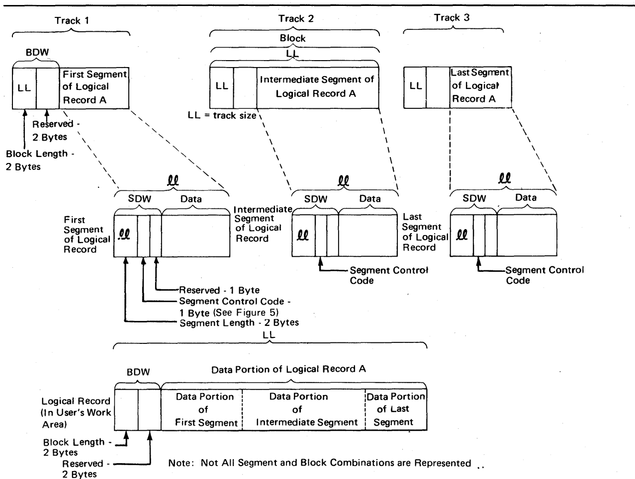
Figure 6. Spanned Variable-Length Records for BDAM Data Sets
