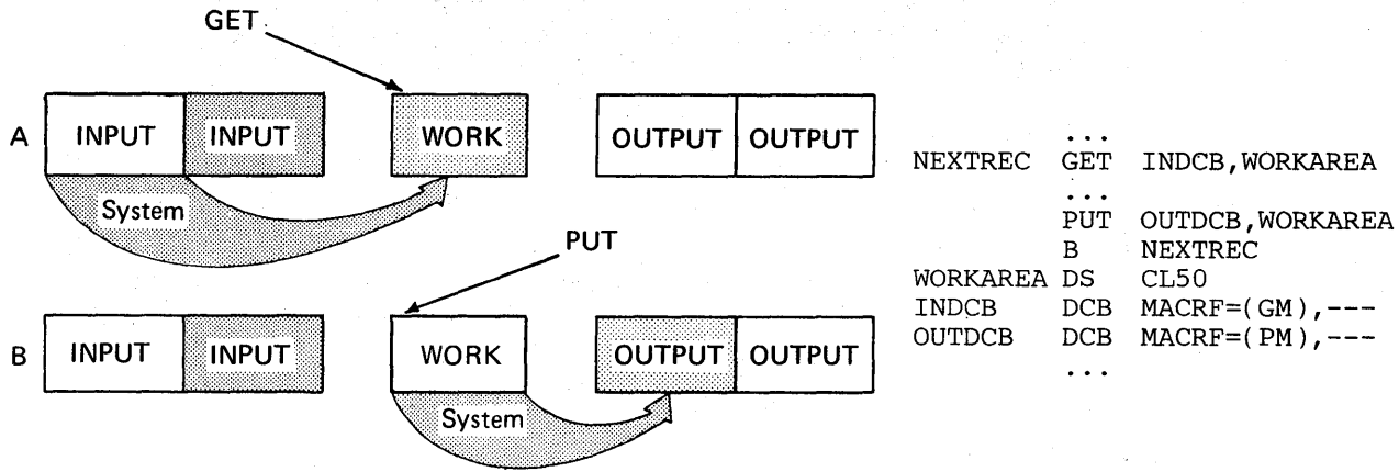
Figure 34. Simple Buffering with MACRF=GM and MACRF=PM
