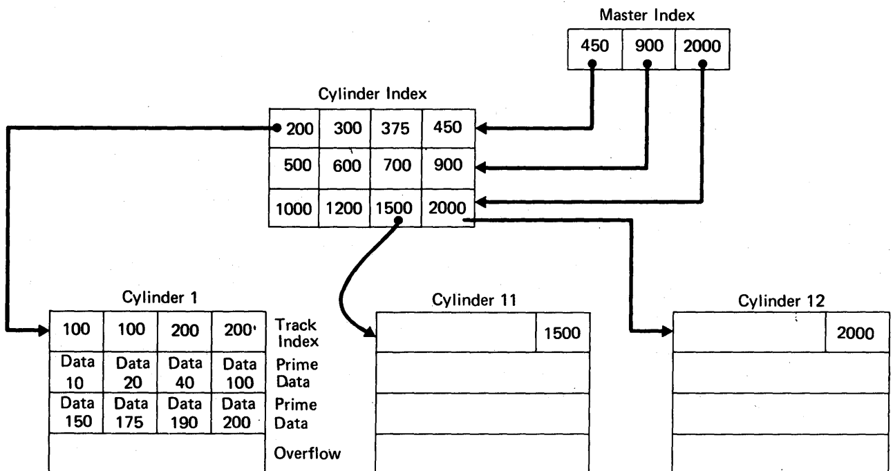
Figure 55. Indexed Sequential Data Set Organization
