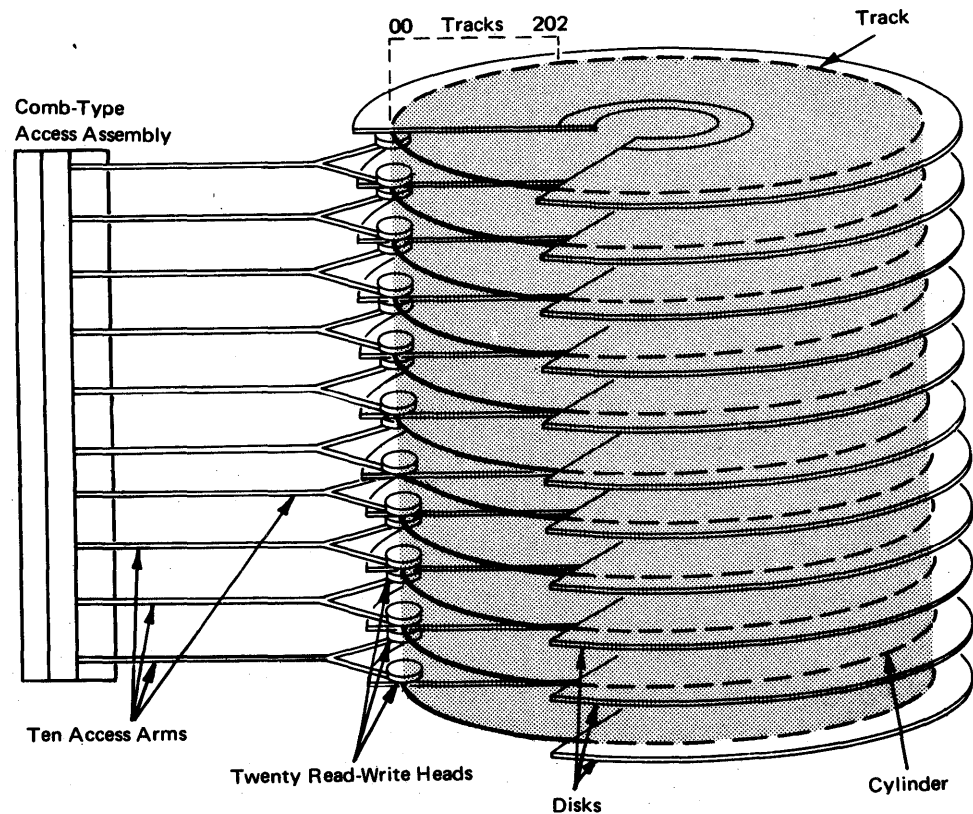
Figure 10. 2316 Disk Pack
