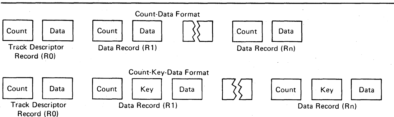
Figure 11. Direct-Access Volume Track Formats
