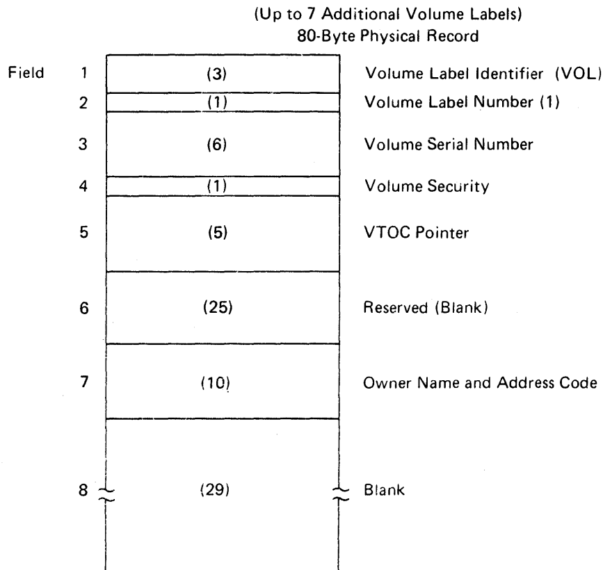
Figure 72. Initial Volume Label
