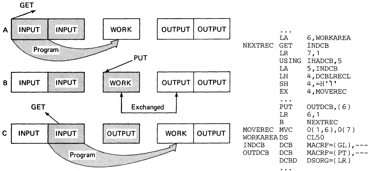
Figure 39. Exchange Buffering with MACRF=GL and MACRF=PT
